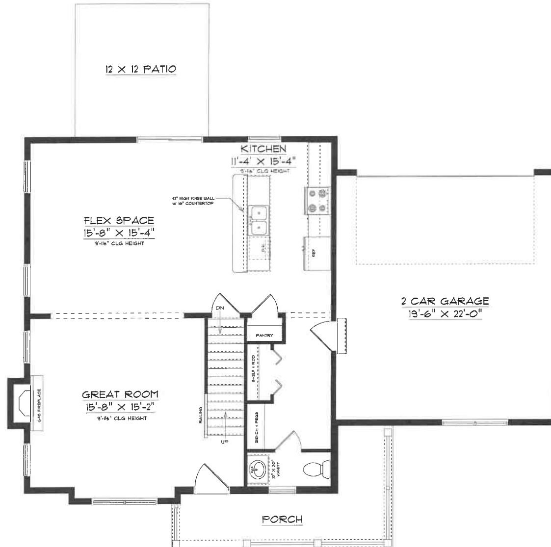
FIRST FLOOR PLAN SCALE: 3/16" = 1'-0"
